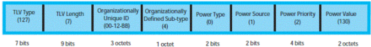
Figure 25. Extended Power via MDI TLV
