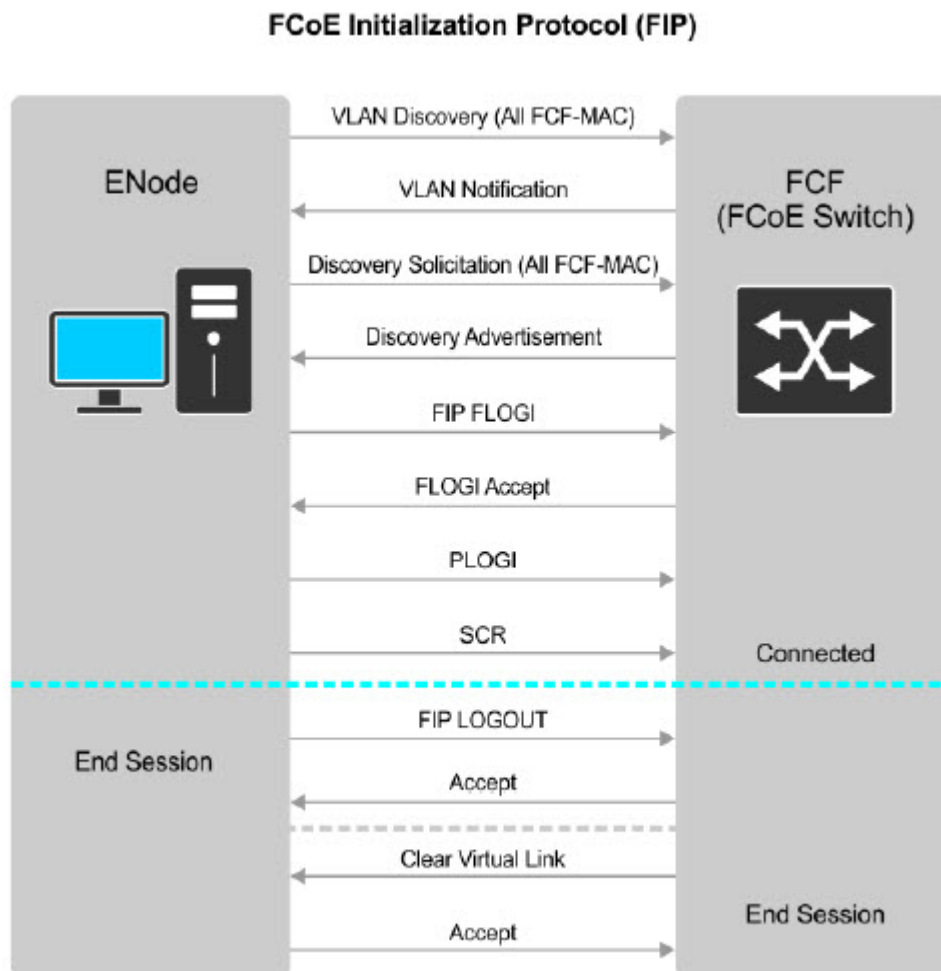
Figure 7. FIP discovery and login between an ENode and an FCF
