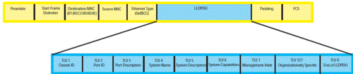
Figure 20. LLDPDU Frame
