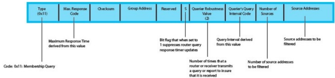
Figure 11. IGMP version 3 Membership Query Packet Format
