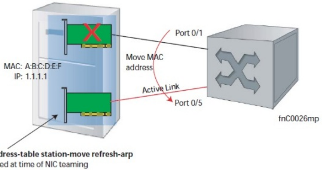
Figure 18. MAC Address Station Move
