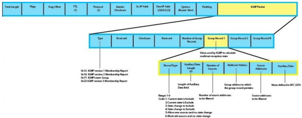
Figure 12. IGMP version 3 Membership Report Packet Format
