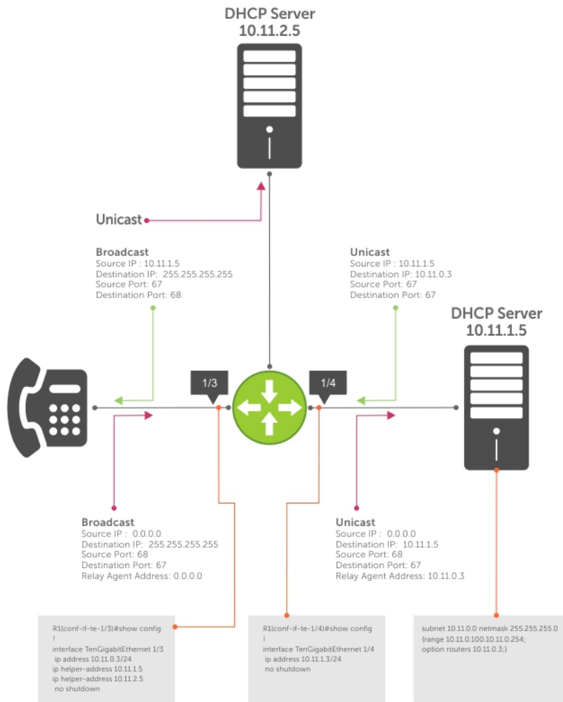
Figure 5. Assigning Network Parameters using DHCP
