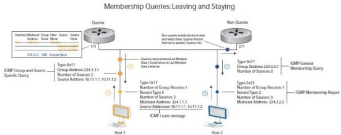
Figure 14. IGMP Membership Queries: Leaving and Staying in Groups
