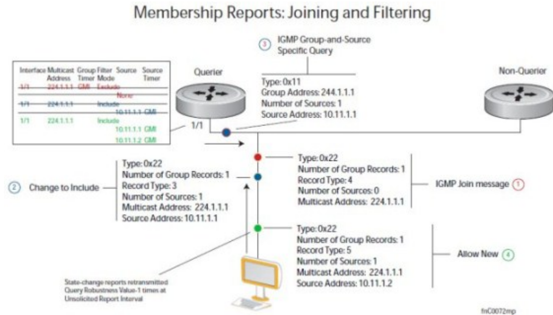
Figure 13. IGMP Membership Reports: Joining and Filtering
