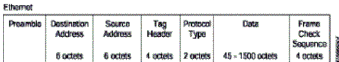
Figure 15. Tagged Frame Format
