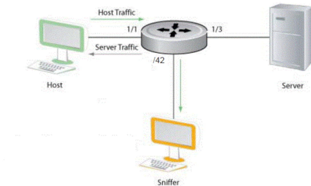
Figure 27. Port Monitoring Example
