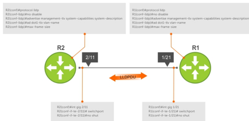
Figure 21. Configuring LLDP
