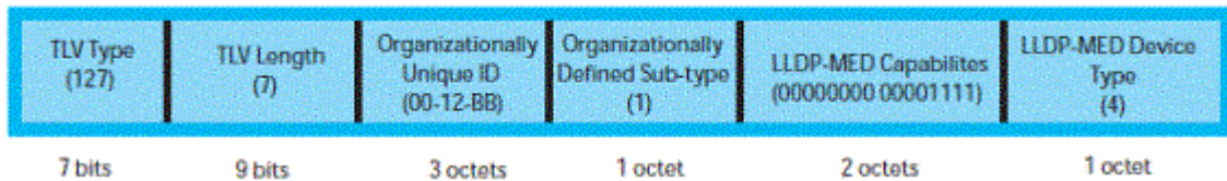
Figure 23. LLDP-MED Capabilities TLV
