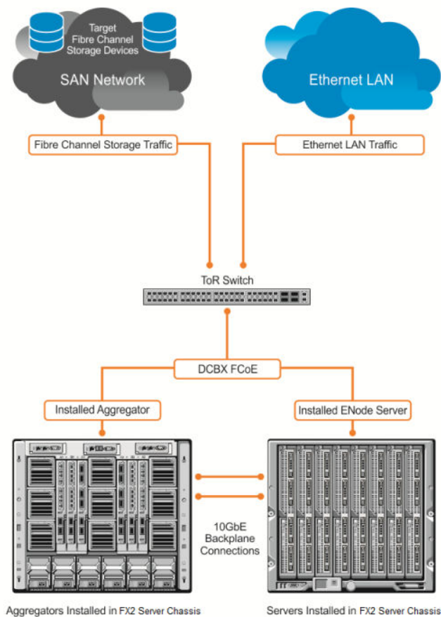
Figure 8. FIP Snooping on an Aggregator
