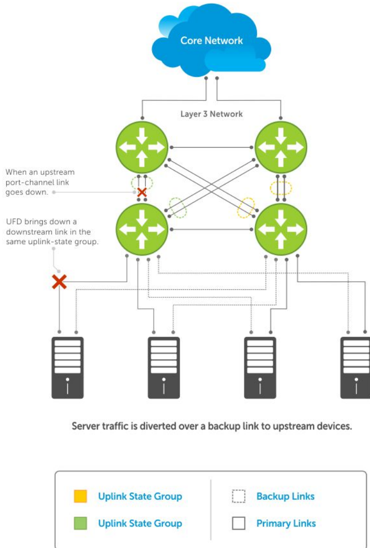
Figure 29. Uplink Failure Detection Example
