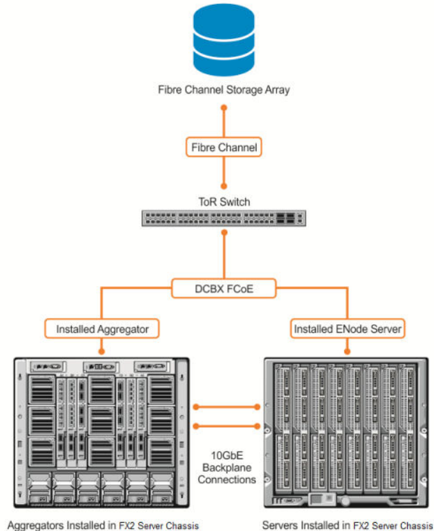
Figure 9. FIP Snooping on an Aggregator
