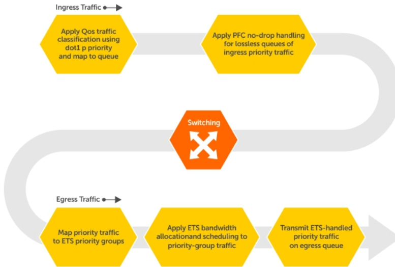
Figure 3. DCB PFC and ETS Traffic Handling
