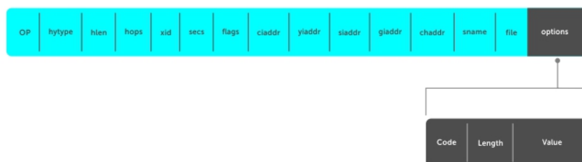
Figure 6. DHCP packet Format
