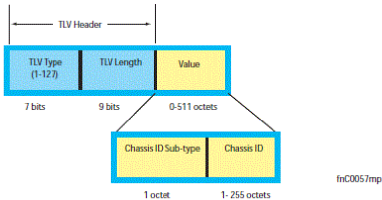
Figure 19. Type, Length, Value (TLV) Segment
