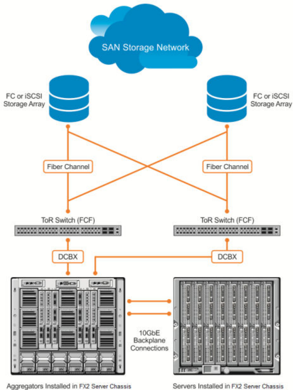
Figure 4. DCBx Sample Topology
